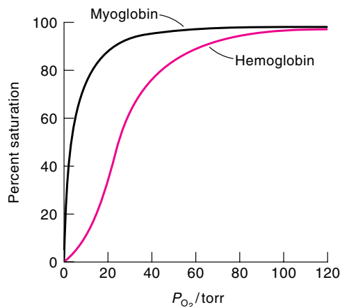
Figure 10.17 Oxygen saturation curves for myoglobin and hemoglobin.
